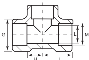
3000 lb. SOCKET WELD TEE
